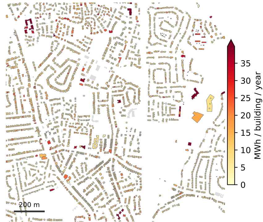
(a) Useful space heat
