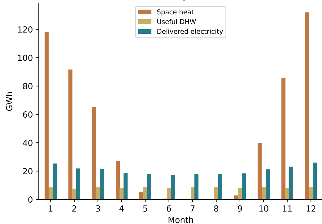
(a) Monthly demand
