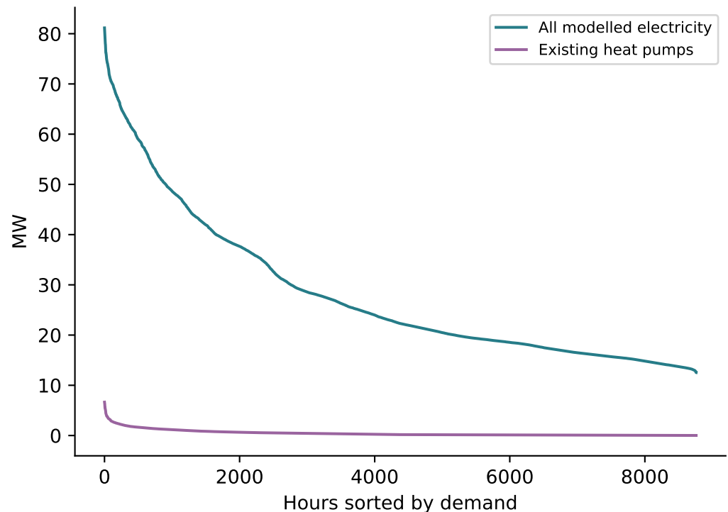
(b) Modelled load-duration curves
