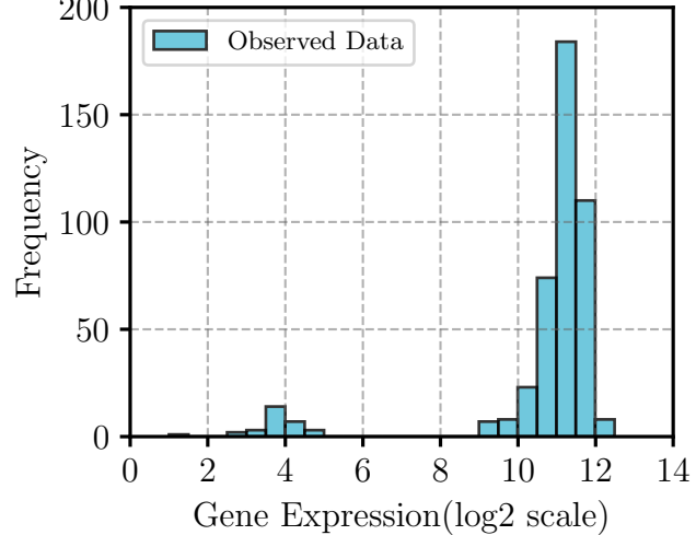
Observed Data Histogram
