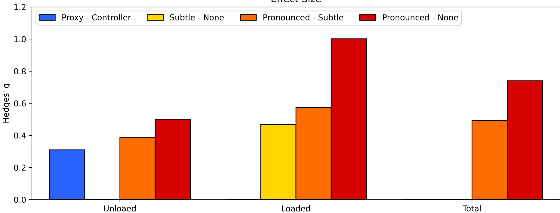
Effect Size
