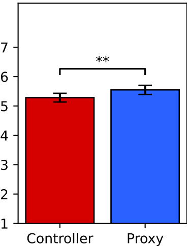
Input Modality
