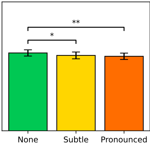
Pseudo-Haptics Intensity
