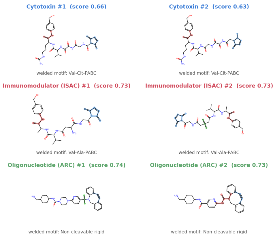
Figure 6: Example generated (trial) linkers from the pool, two per payload class. Every molecule is a real REINVENT design carrying its literature-derived motif by construction; handle (blue), scissile bond (red) and spacer (green) are SMARTS-detected. The ARC designs (bottom) carry the rigid non-cleavable DBCO cap—no scissile bond—while the cytotoxin/ISAC designs carry cleavable Val-Cit/Val-Ala dipeptides.
