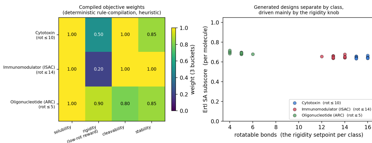
Figure 3: The rules steer the chemistry. Left: the compiled objective weights—a deterministic rule-compilation (a heuristic keyed by the agent’s derived category, effectively three buckets, not continuously tuned). The “rigidity” term rewards fewer rotatable bonds; the real separator is the per-class rotatable-bond setpoint (rot ≤ 5/10/14), shown by each class. ISAC’s stability weight is floored to paramount by the low-evidence safety gate. Right: the generated designs separate by class, driven mainly by the rigidity setpoint (x); y is the per-molecule Ertl SA subscore (a real quantity, not jitter).
