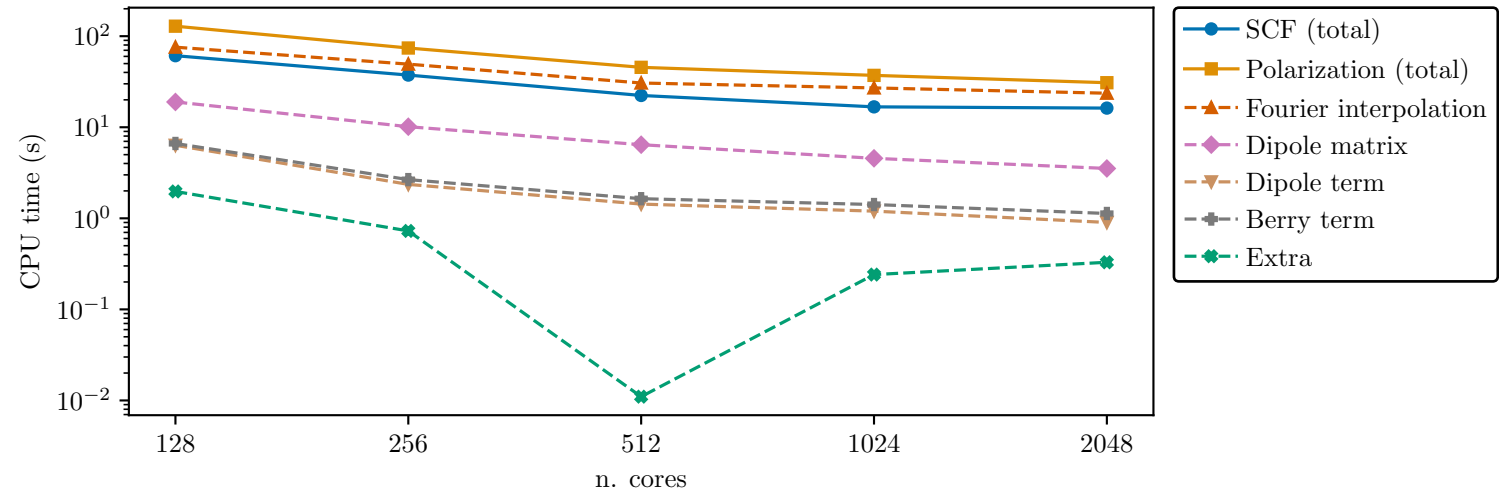
revPBE, 128 water molecules
