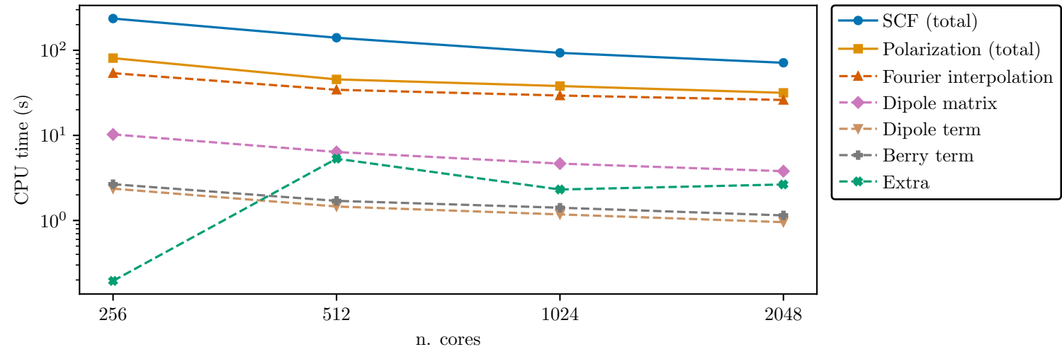
revPBE0, 128 water molecules
