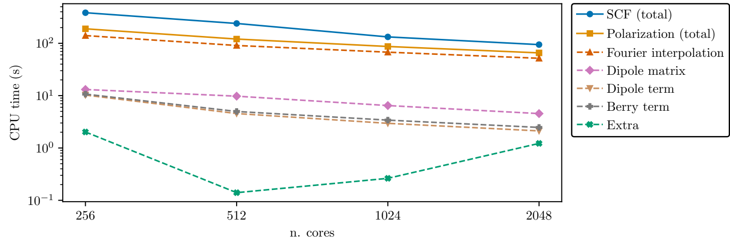
revPBE0, 196 water molecules
