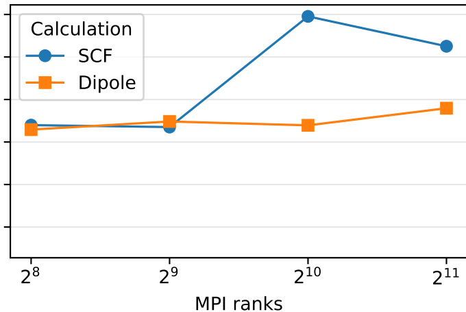
196 water molecules
