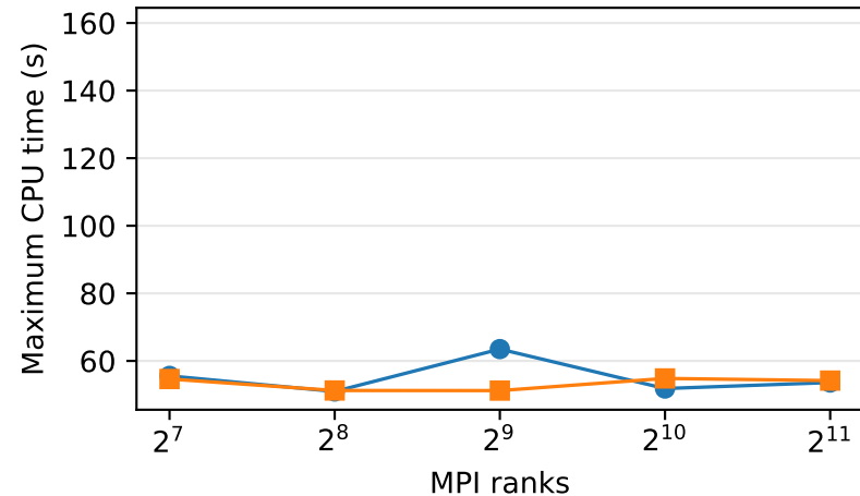
128 water molecules
