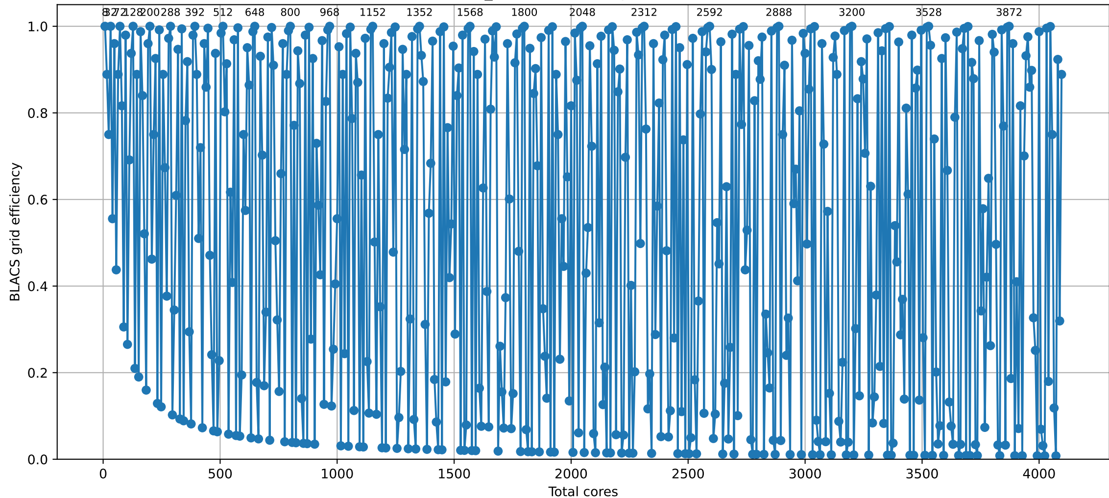
BLACS Grid Efficiency n_basis=10192, k-points=8
