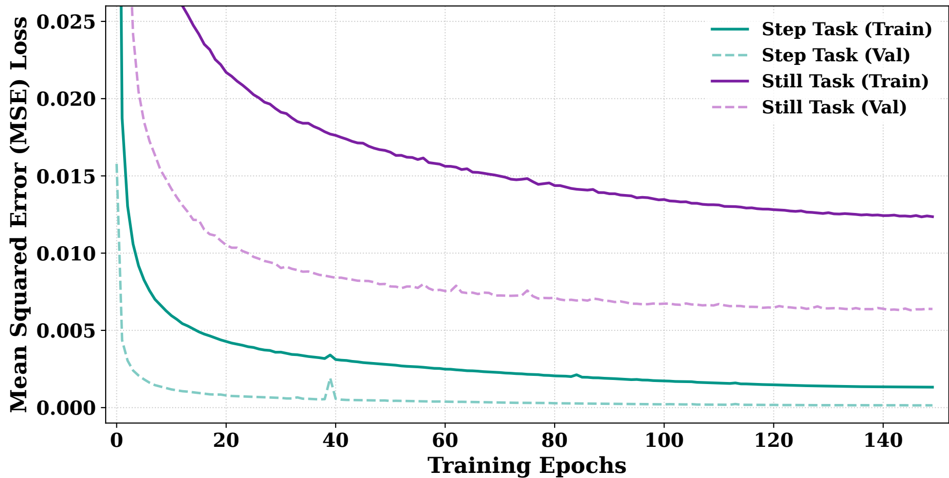
Loss Evolution
