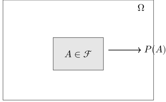
Figure 1: Structure of a probability space (\Omega, \mathcal{F}, P) . The outer rectangle represents the sample space \Omega , normalized so that its total area equals 1. The shaded region is an event A \in \mathcal{F} , and P(A) is the ratio of the shaded area to the total area of \Omega . The \sigma -algebra \mathcal{F} is not depicted as a region but is understood as the family of all subsets of \Omega — such as A — to which P can be legitimately assigned.
