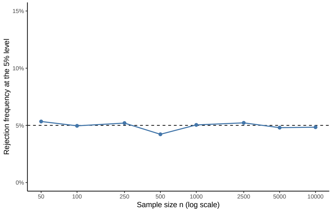
Size of Hansen's J overidentification test ( df = 1 )
