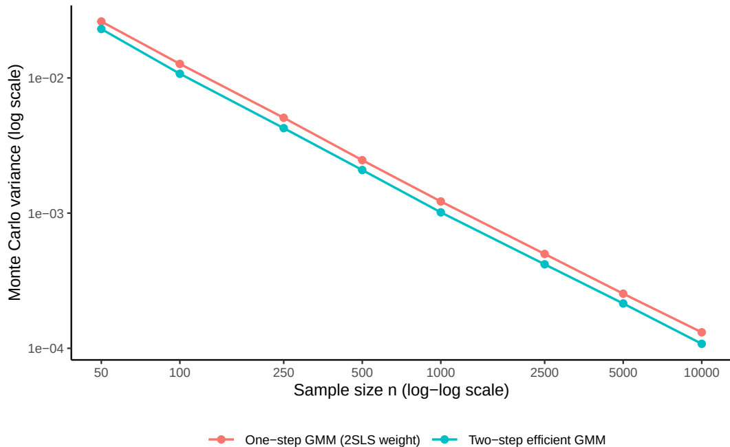
Efficiency: two-step GMM attains lower sampling variance
