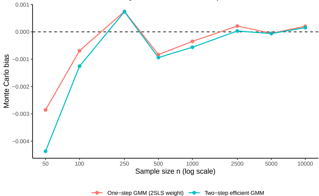
Consistency: bias of the GMM slope estimator
