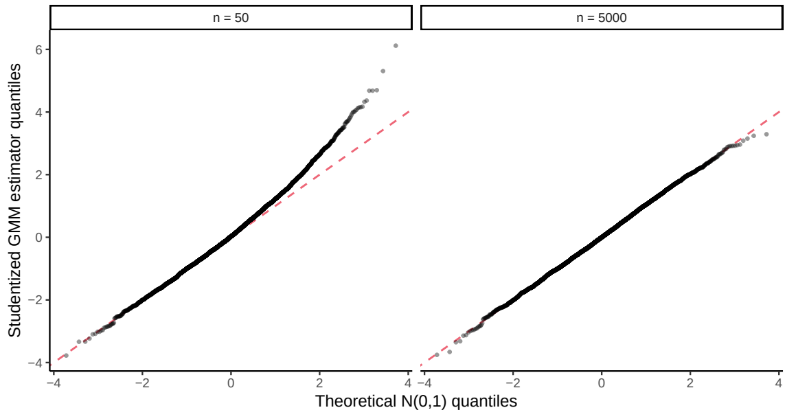
QQ-plot of the studentized two-step GMM estimator
