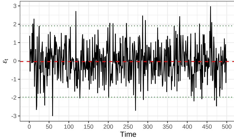
Figure 3: Gaussian white noise (i.i.d. N(0,1) )
