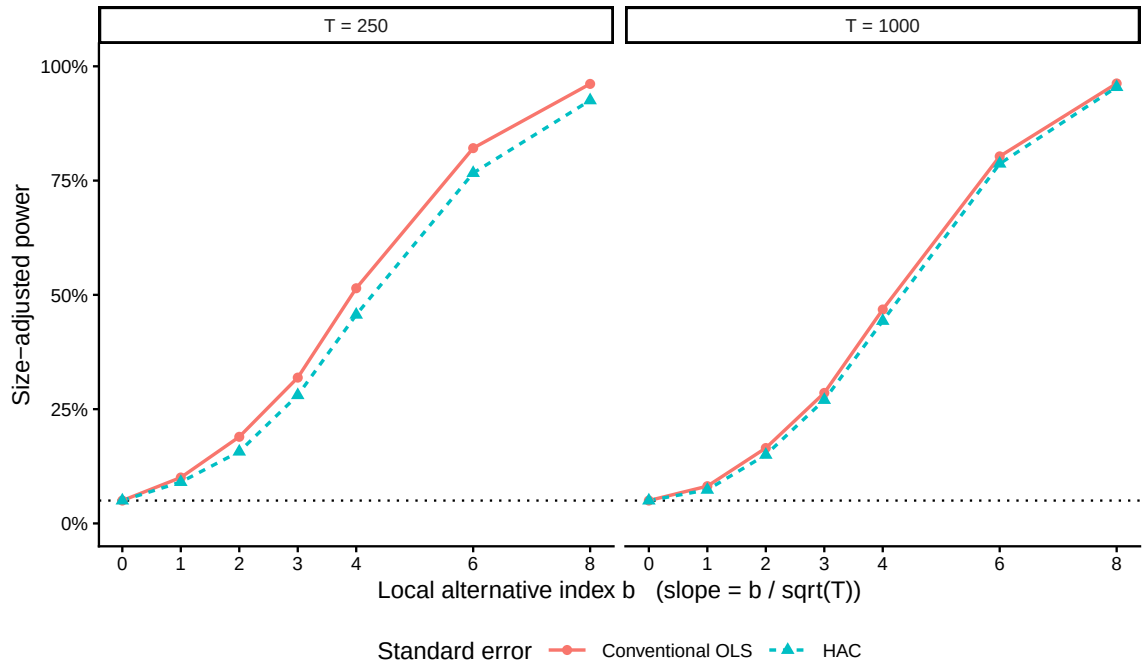
Size-adjusted local power, AR(1) pair with \phi = 0.8
