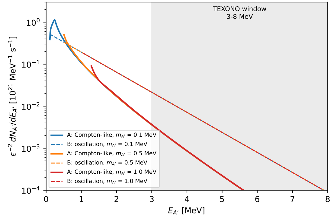
A' spectrum at the reactor: 1 GW, Park spectrum, \varepsilon = 1
