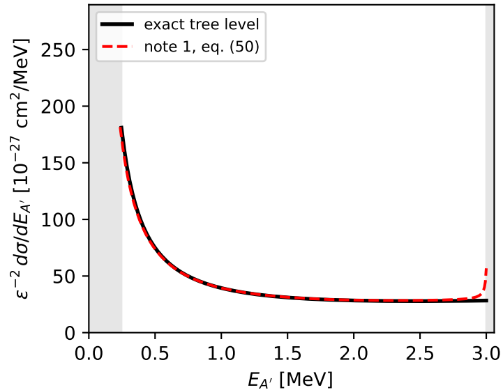
E_\gamma = 3.0 \text{ MeV}, m_{A'} = 0.1 \text{ MeV}
