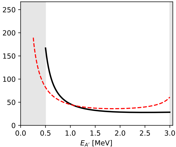
E_\gamma = 3.0 \text{ MeV}, m_{A'} = 0.5 \text{ MeV}
