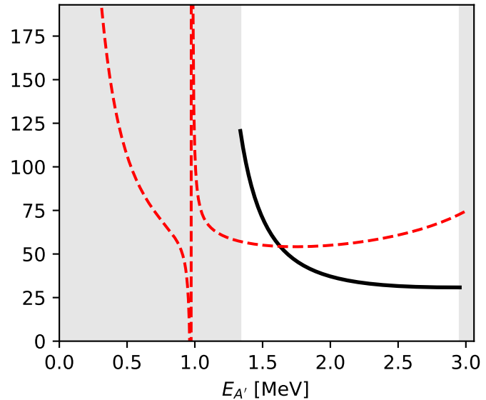
E_\gamma = 3.0 \text{ MeV}, m_{A'} = 1.0 \text{ MeV}
