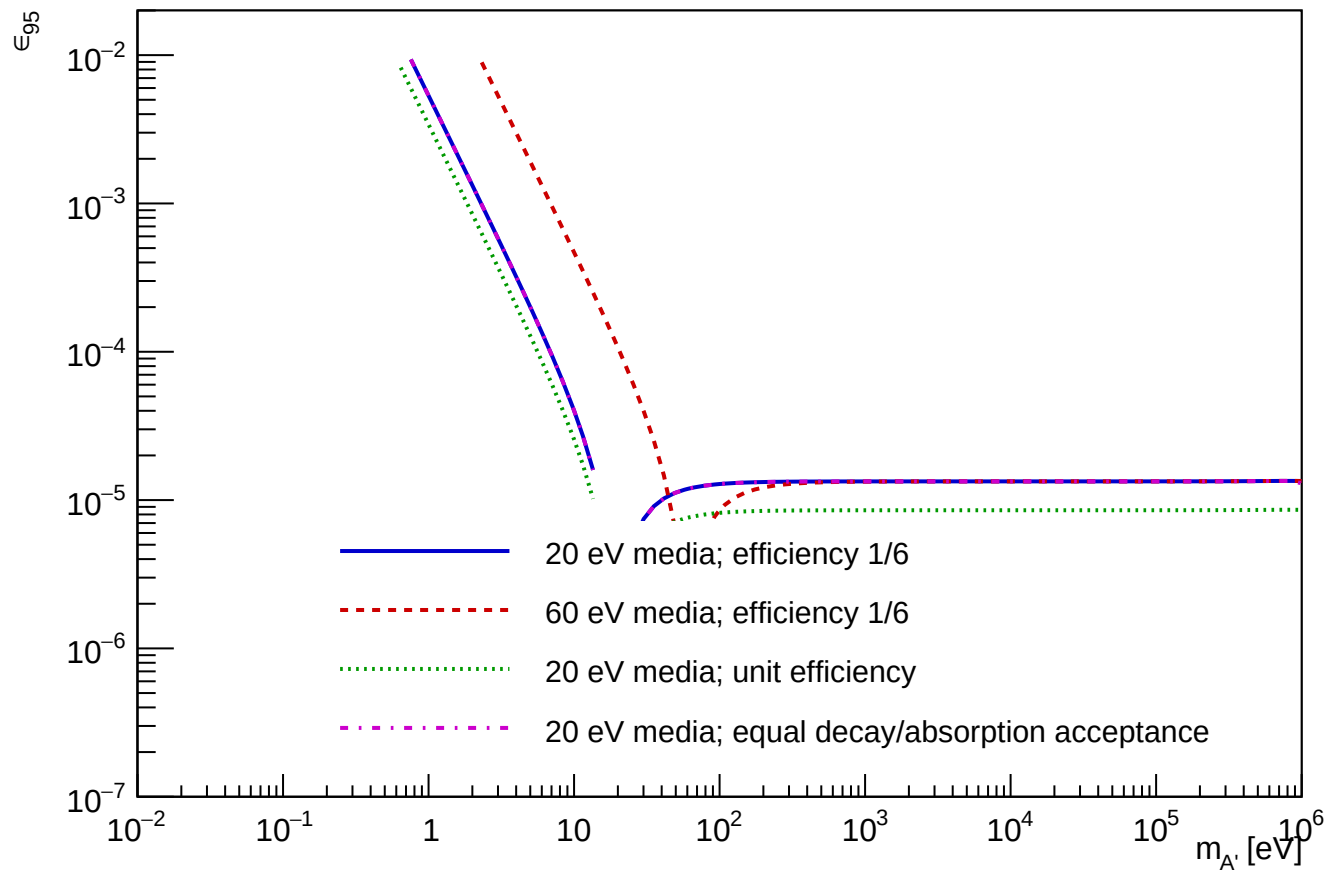
TEXONO: one-sided Gaussian 95% CL, conditional response
