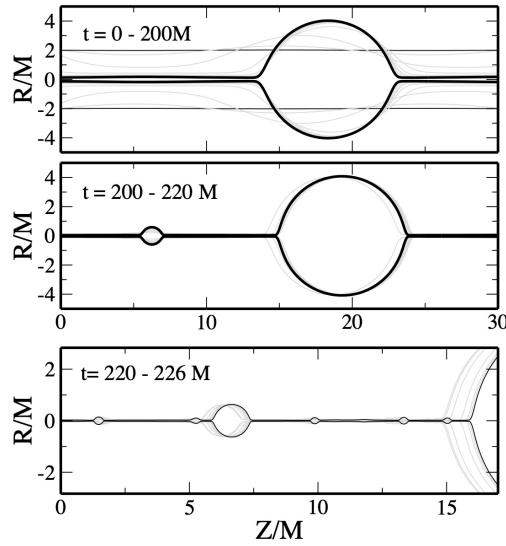
Figure 6: Position of apparent horizon in numerical simulation of Gregory-Laflamme instability. Image credit: [18]
