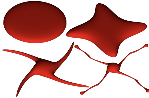
Figure 10: Numerical evolution of m -bar instability of unstable BH for m = 4 . Image credit: [15]
