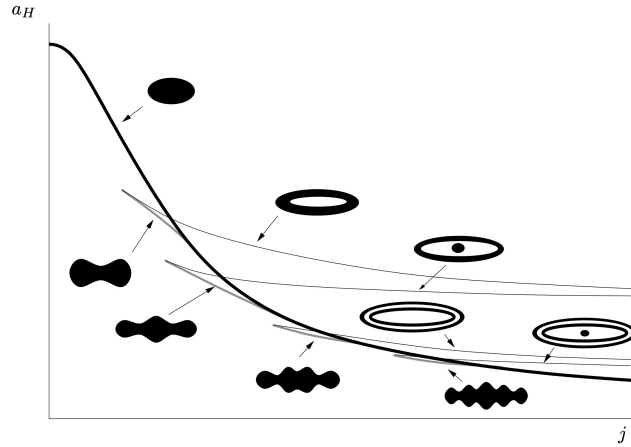
Figure 22: Proposed phase diagram for singly spinning black objects in d \geq 6 . Image credit: [51]
