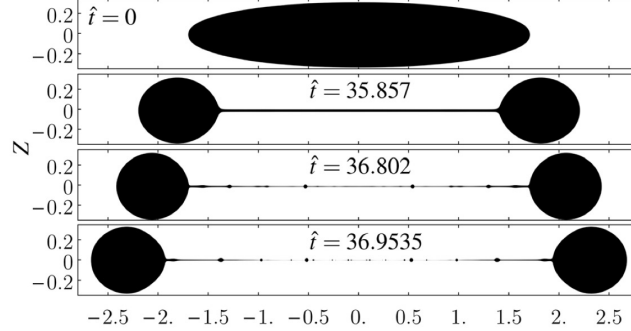
Figure 16: Simulation of apparent horizon (cross-section shown) dynamics for ultraspinning instability. Image credit: [35]
