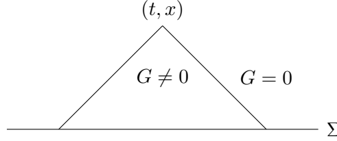
Figure 2: Past light cone starting on (t, x) .
