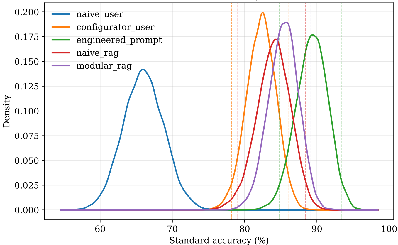
Bootstrap distribution of standard accuracy (10 000 cluster resamples)
