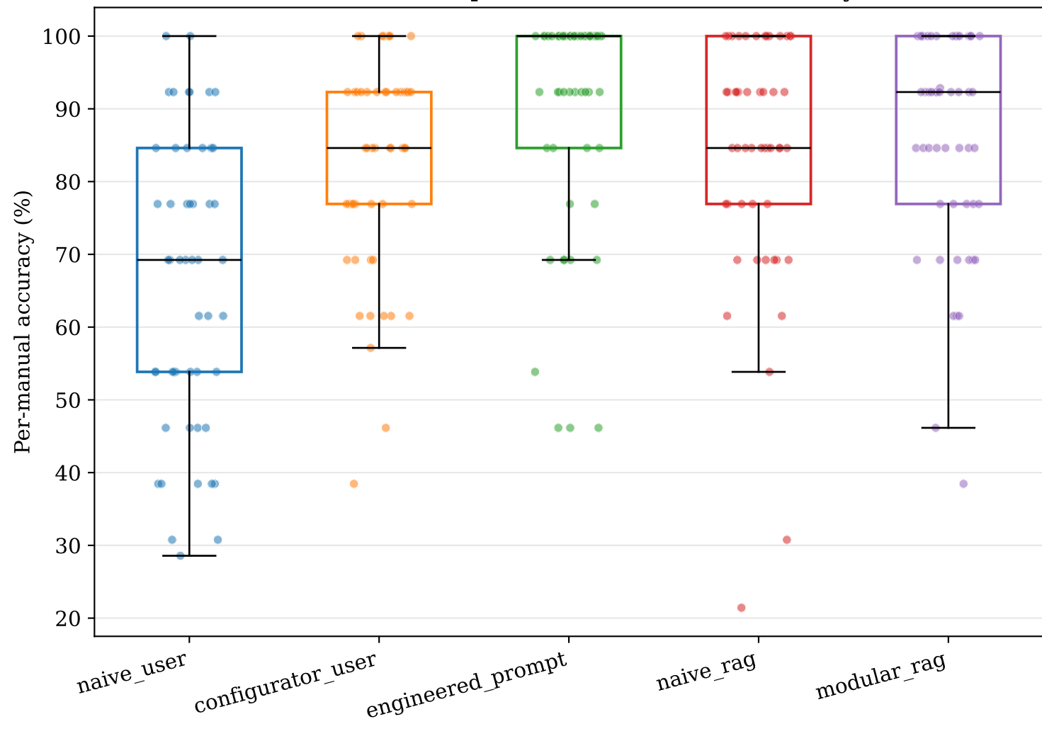
Distribution of per-manual standard accuracy
