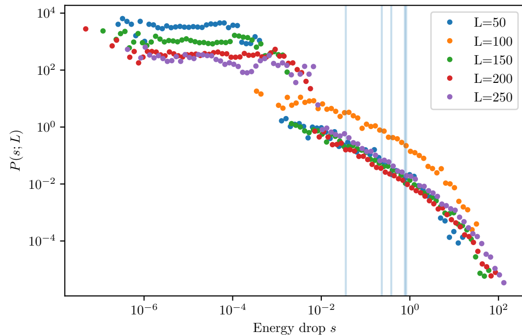
First-order elastic continuation - post-yield Per-size global_min xmin (vertical lines)
