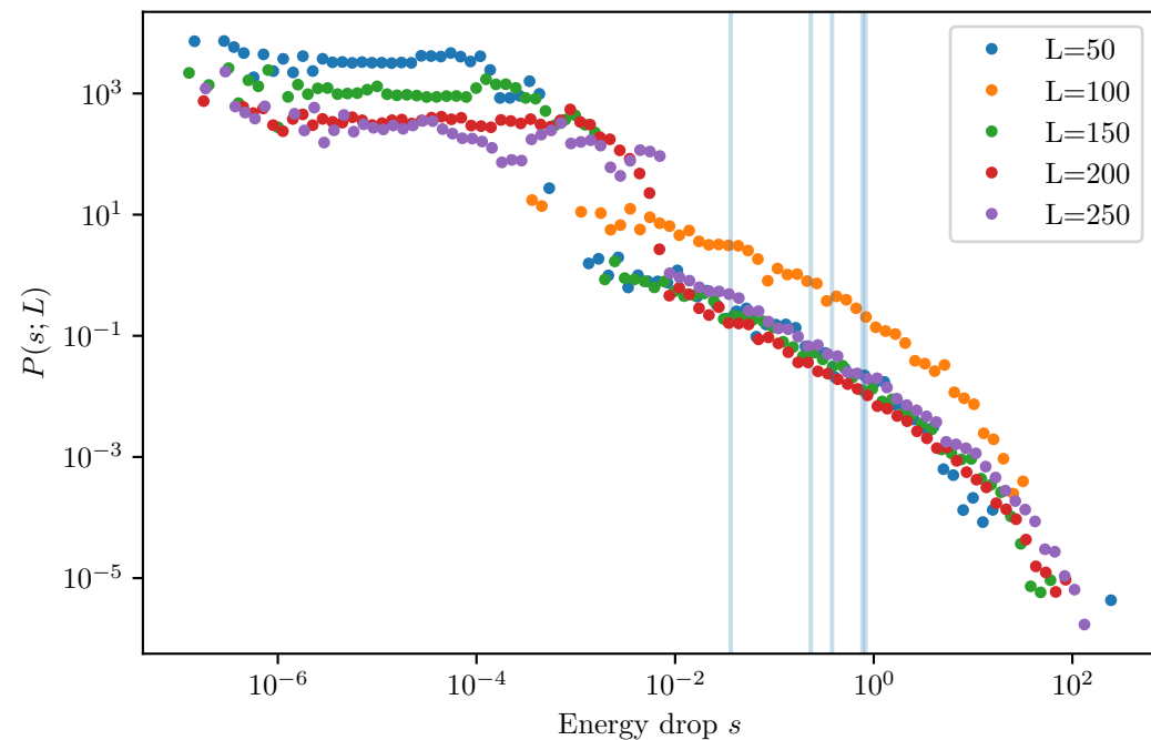
Second-order elastic continuation - post-yield Per-size global_min xmin (vertical lines)
