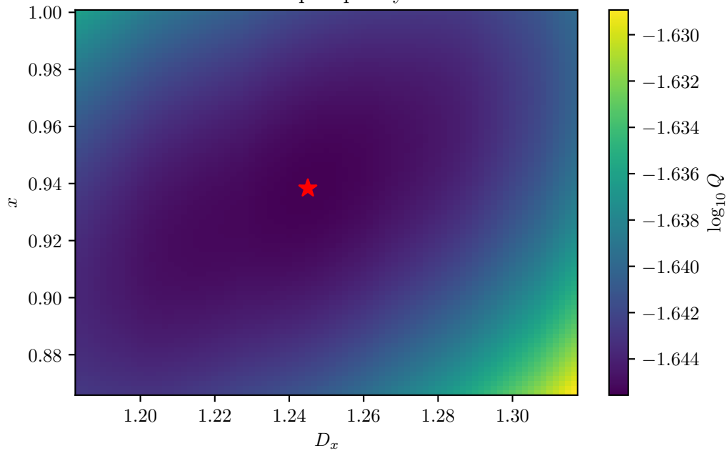
Collapse quality
