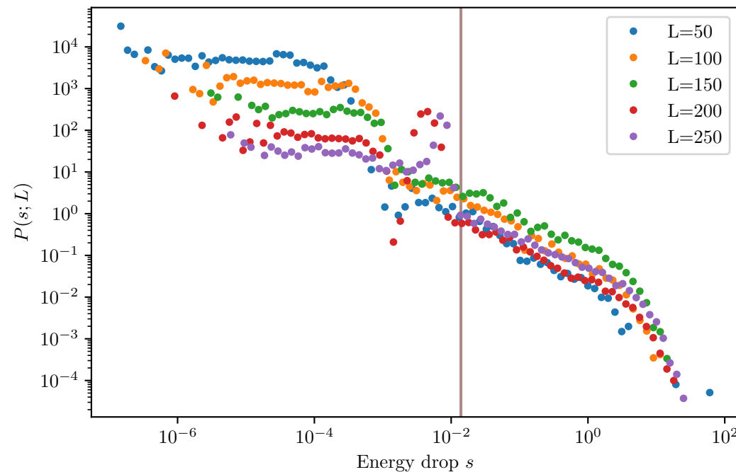
First-order elastic continuation - pre-yield Shared xmin=1.388e-02 from L=250 (plateau)
