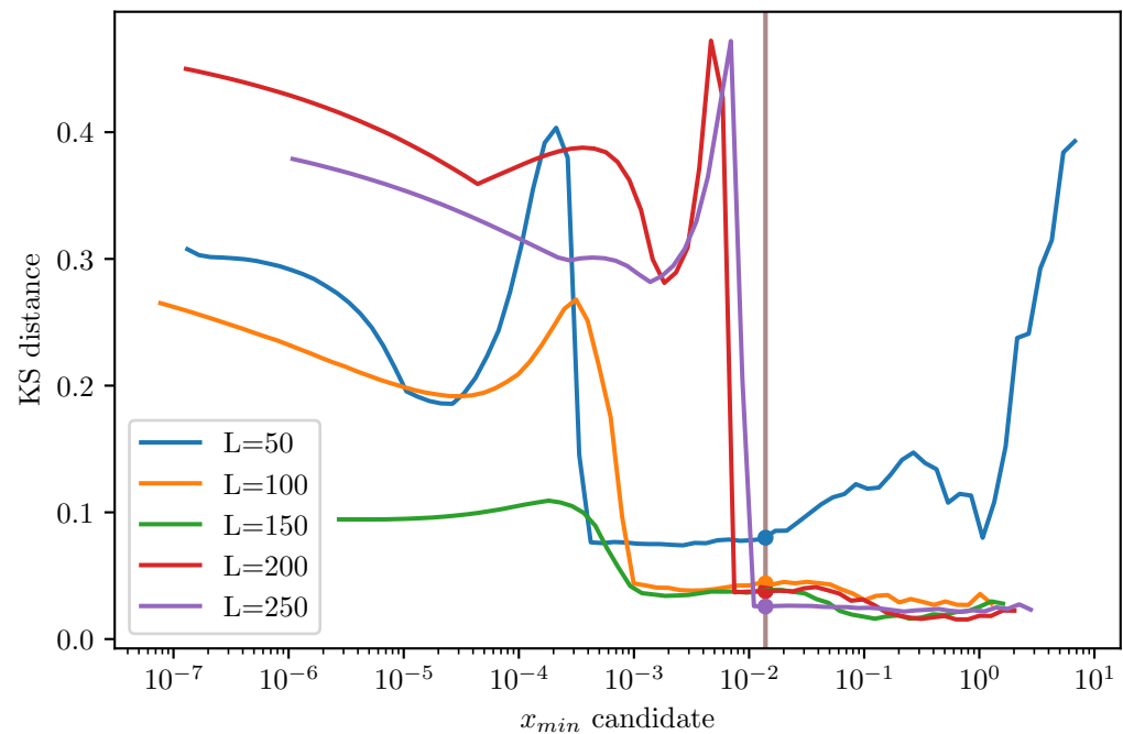
First-order elastic continuation - pre-yield Shared xmin=1.388e-02 from L=250 (plateau)
