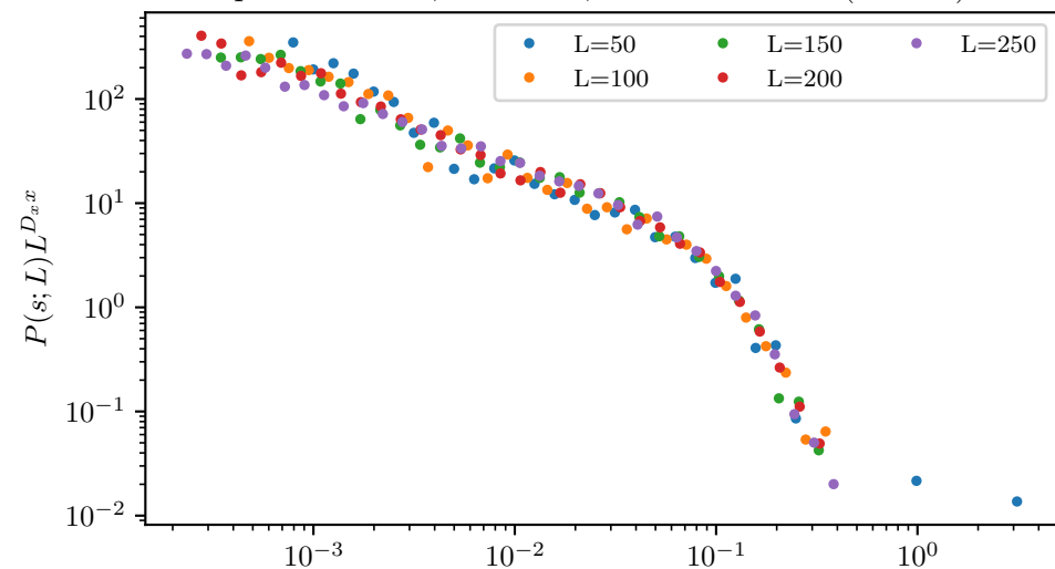
First-order elastic continuation pre: x=1.080 , D=0.802 , x_{\min}=1.39\text{e-}02 ( L=250 )
