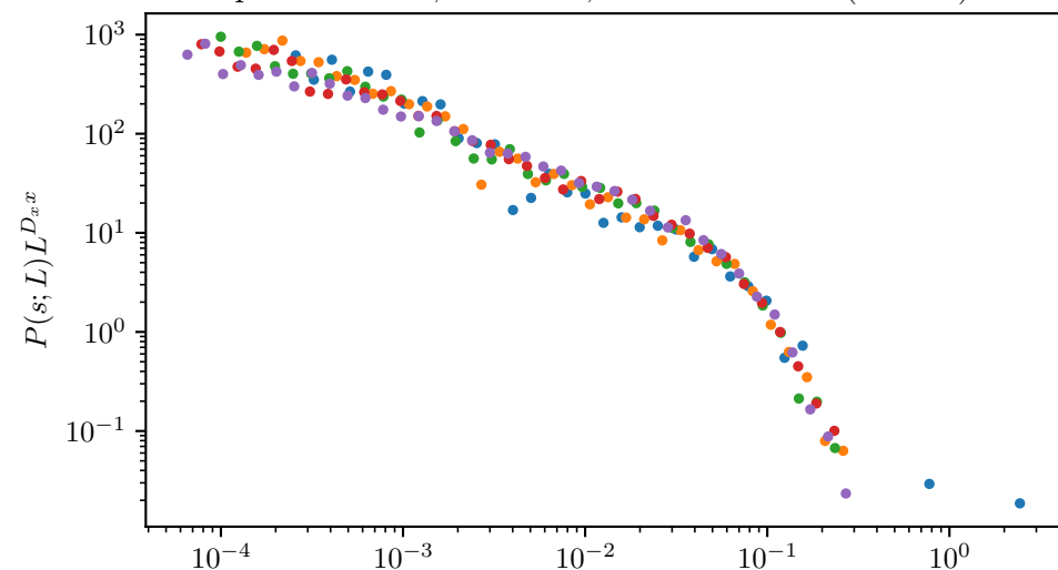
Affine initial-guess energy pre: x=0.737 , D=0.500 , x_{\min}=1.25\text{e-}05 ( L=250 )
