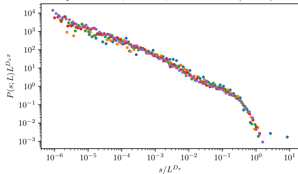
Affine initial-guess energy pre: x=0.737 , D=0.500 , x_{\min}=1.25\text{e-}05 ( L=250 )
