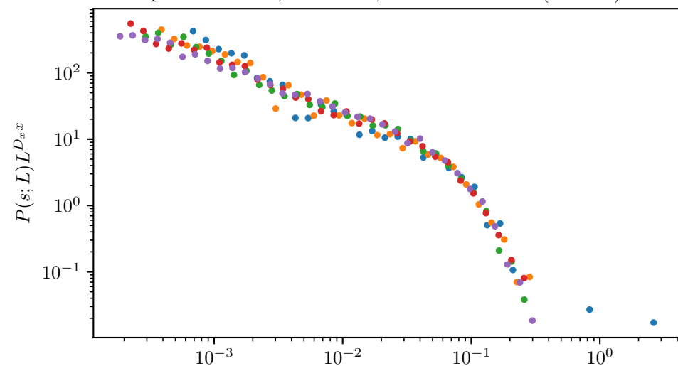
Previous relaxed energy pre: x=1.113 , D=0.820 , x_{\min}=5.35\text{e-}03 ( L=250 )
