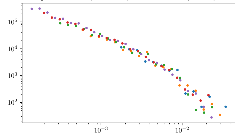
Affine initial-guess energy post: x=0.500 , D=0.372 , x_{\min}=6.44\text{e-}06 ( L=250 )
