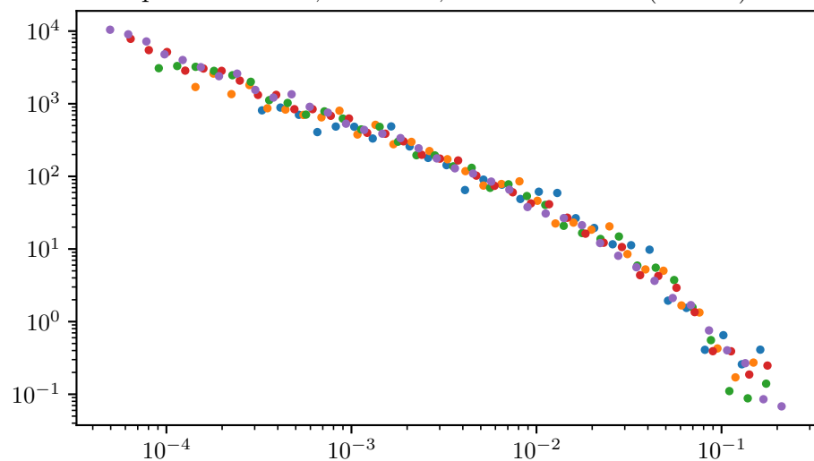
Previous relaxed energy post: x=1.568 , D=1.568 , x_{\min}=7.21\text{e-}01 ( L=250 )
