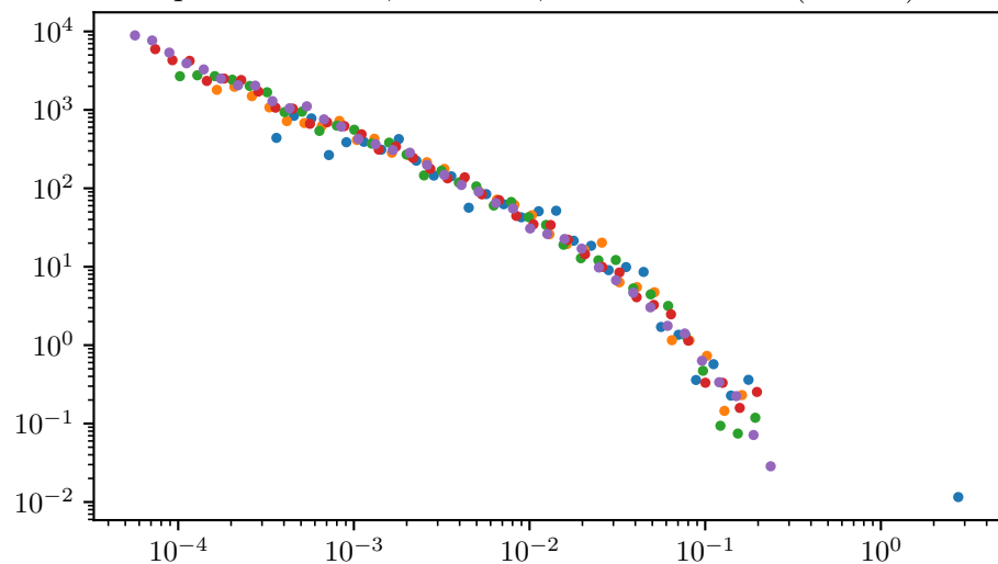
First-order elastic continuation post: x=1.187 , D=1.167 , x_{\min}=2.76\text{e-}02 ( L=250 )
