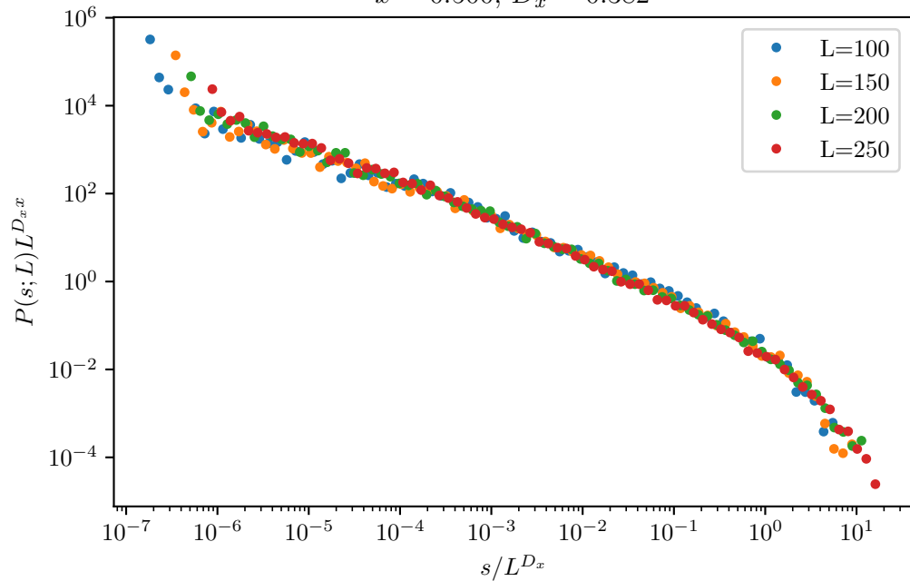
x = 0.500, D_x = 0.382
