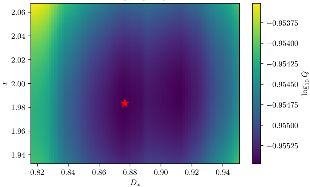
Collapse quality
