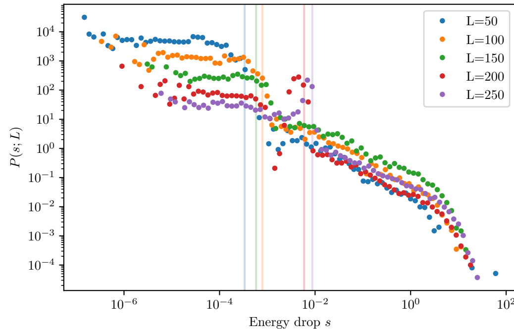
First-order elastic continuation - pre-yield Per-size slope xmin (vertical lines)
