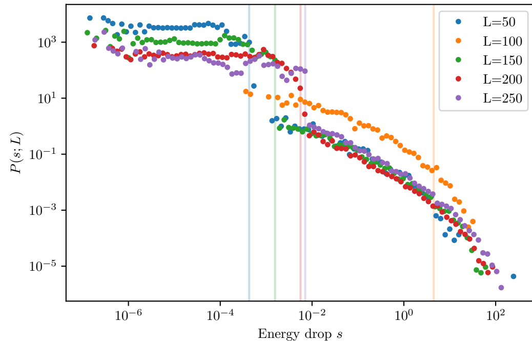
Second-order elastic continuation - post-yield Per-size slope xmin (vertical lines)
