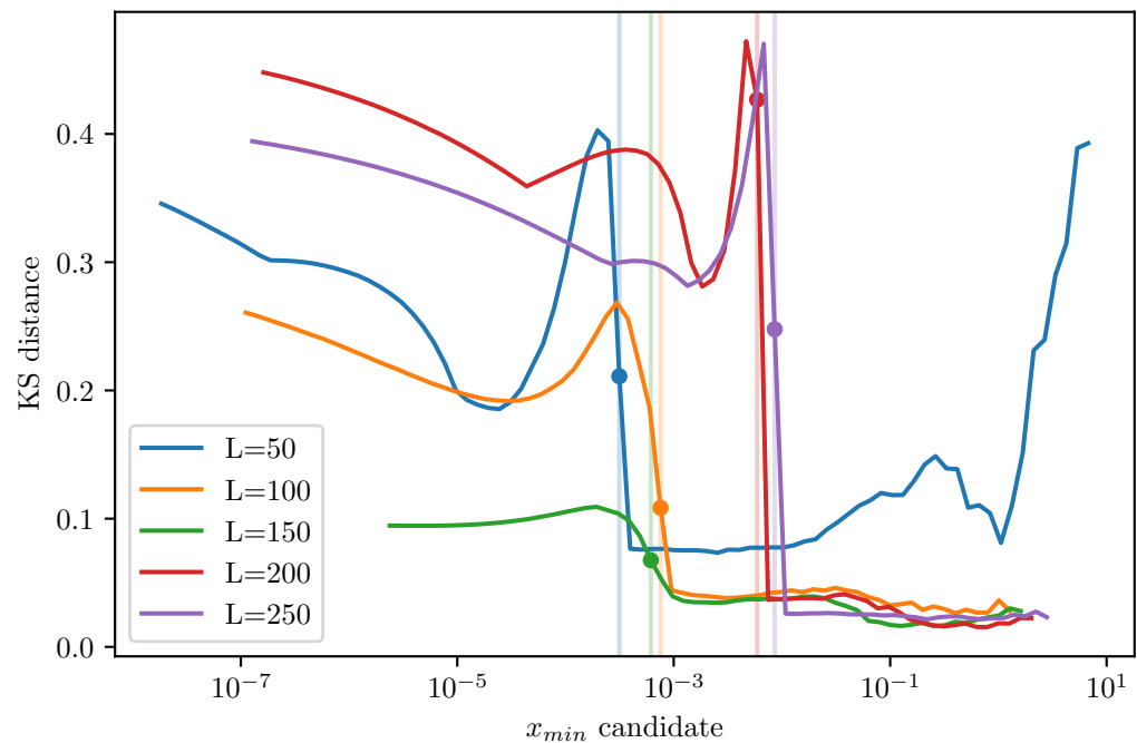
Second-order elastic continuation - pre-yield Per-size slope xmin (vertical lines)
