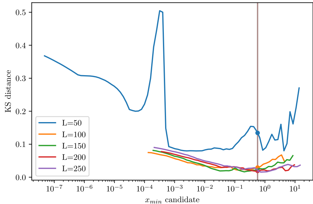
Previous relaxed energy - post-yield Shared xmin=5.710e-01 from L=250 (slope)
