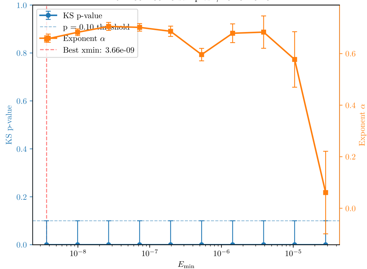
FIRE 200x200 10 samples \gamma : 0.15 - 0.40
