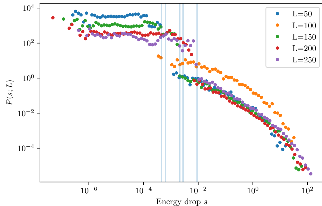
First-order elastic continuation - post-yield Per-size plateau xmin (vertical lines)
