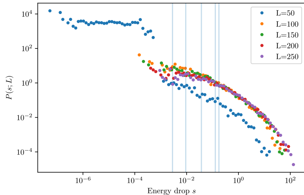
Previous relaxed energy - post-yield Per-size plateau xmin (vertical lines)
