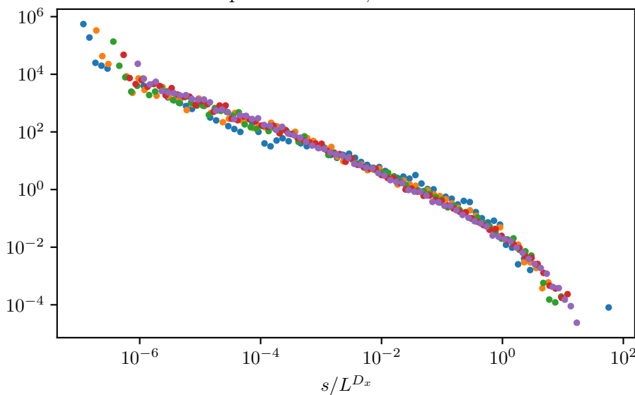
Affine initial-guess energy post: x=0.500 , D=0.372
