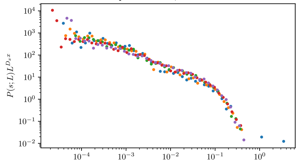
Affine initial-guess energy pre: x=0.500 , D=2.250
