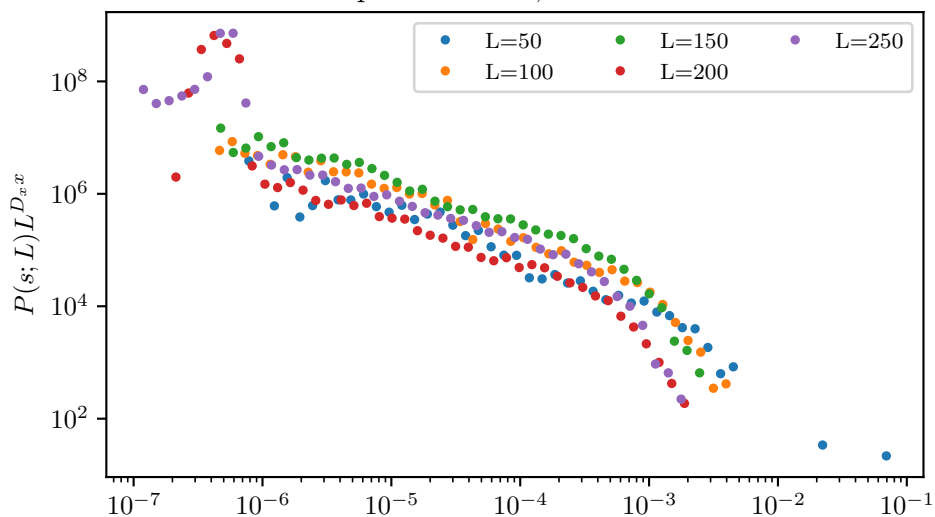
First-order elastic continuation pre: x=1.590 , D=1.737
