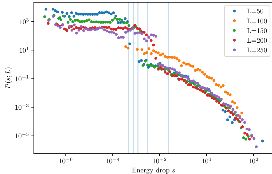
Second-order elastic continuation - post-yield Per-size plateau xmin (vertical lines)
