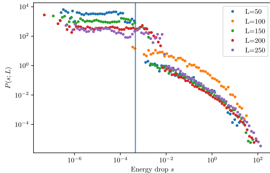
First-order elastic continuation - post-yield Shared xmin=4.541e-04 from L=250 (plateau)
