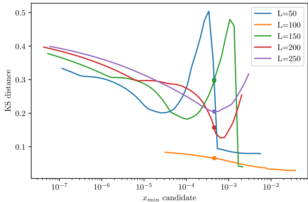
First-order elastic continuation - post-yield Shared xmin=4.541e-04 from L=250 (plateau)
