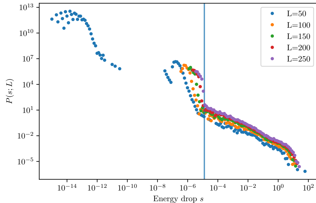
Affine initial-guess energy - pre-yield Shared xmin=1.275e-05 from L=250 (plateau)
