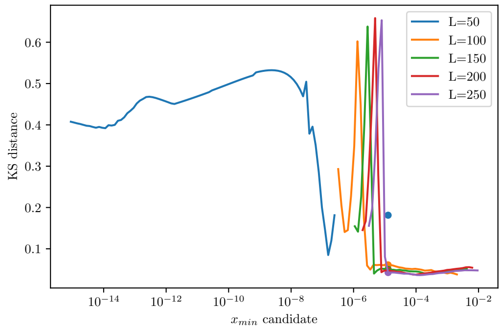
Affine initial-guess energy - pre-yield Shared xmin=1.275e-05 from L=250 (plateau)
