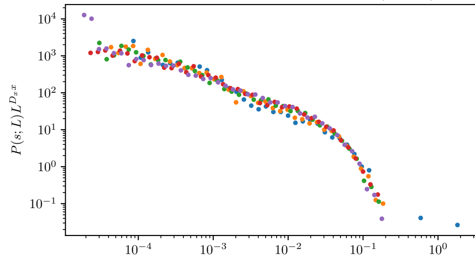
Affine initial-guess energy pre: x=0.738 , D=0.502 , x_{\min}=1.27\text{e-}05 ( L=250 )
