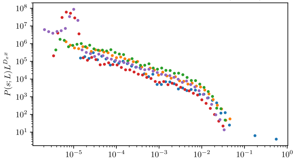
Previous relaxed energy pre: x=1.140 , D=0.895 , x_{\min}=2.36\text{e-}03 ( L=250 )
