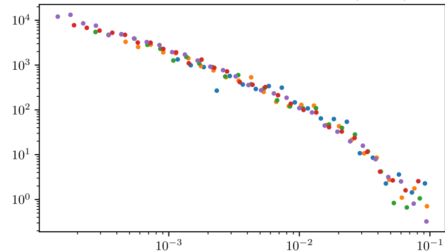
Affine initial-guess energy post: x=0.500 , D=0.255 , x_{\min}=6.43\text{e-}06 ( L=250 )
