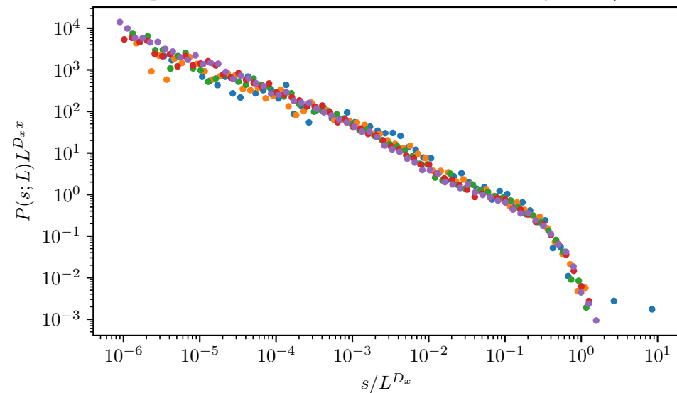
Affine initial-guess energy pre: x=0.738 , D=0.502 , x_{\min}=1.27\text{e-}05 ( L=250 )
