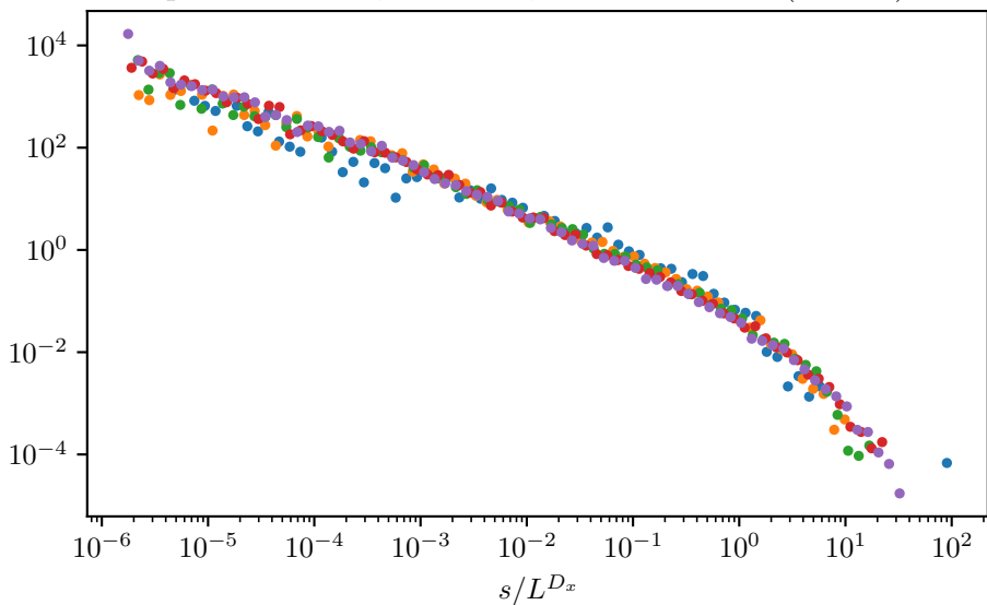
Affine initial-guess energy post: x=0.500 , D=0.255 , x_{\min}=6.43\text{e-}06 ( L=250 )
