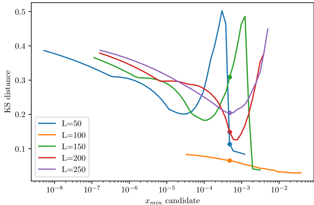
Second-order elastic continuation - post-yield Shared xmin=4.788e-04 from L=250 (plateau)
