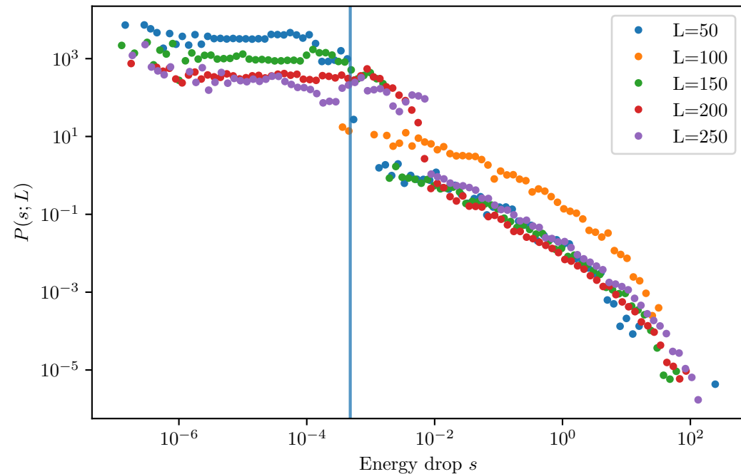
Second-order elastic continuation - post-yield Shared xmin=4.788e-04 from L=250 (plateau)
