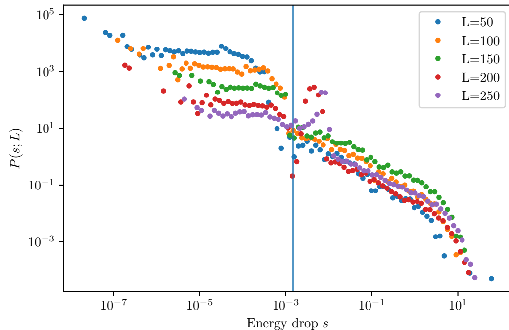
Second-order elastic continuation - pre-yield Shared xmin=1.495e-03 from L=250 (plateau)
