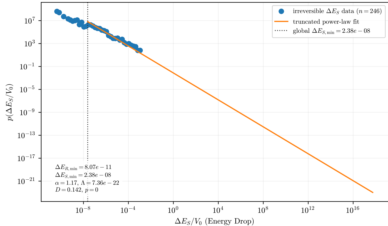
delaunay: post-yield \Delta E_R -classified irreversible \Delta E_S
