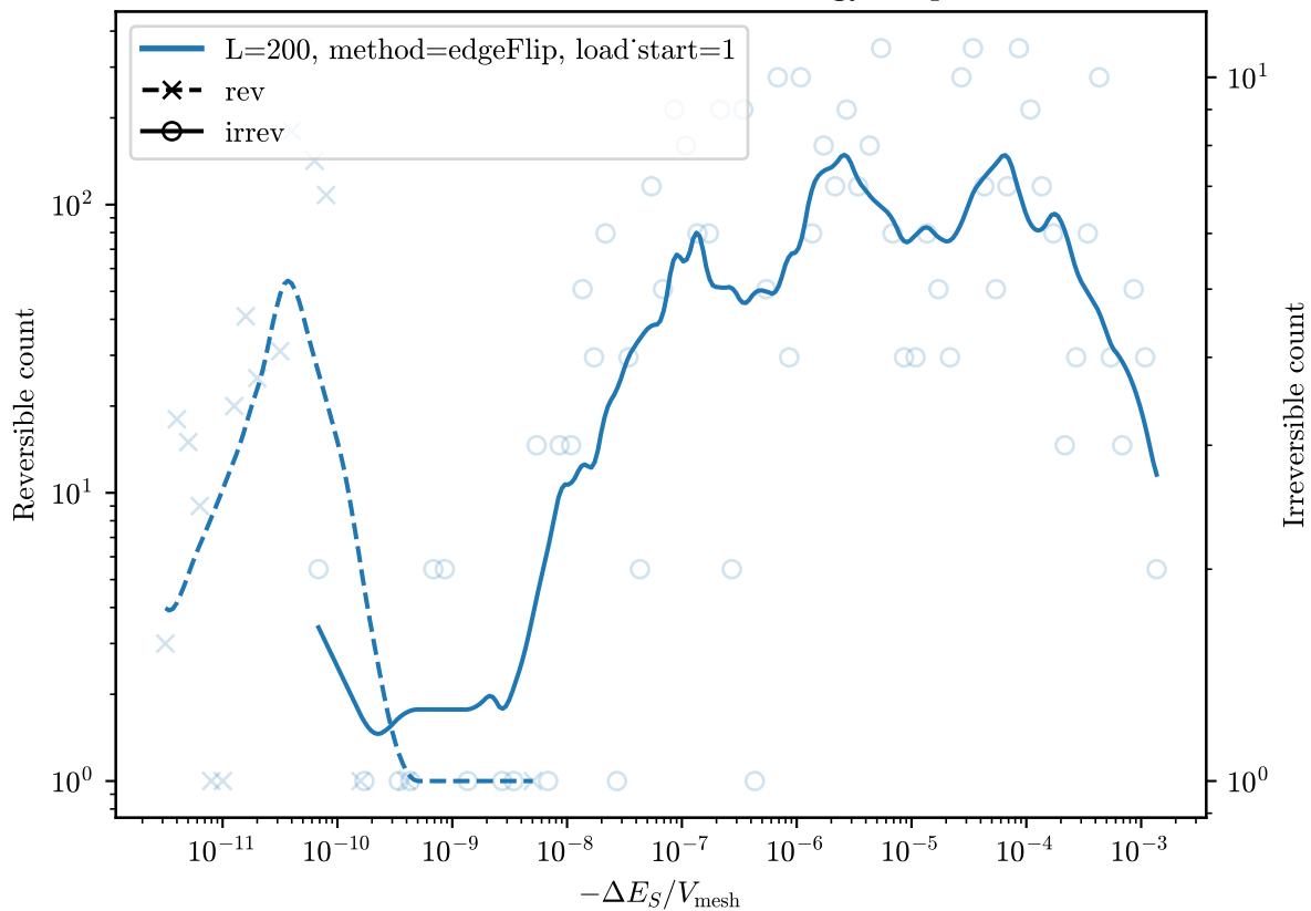
Reversible vs. irreversible energy drops
