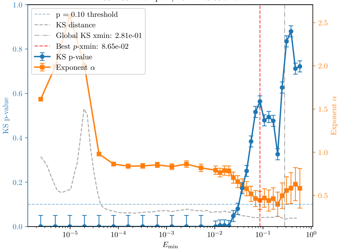
200x200 1 sample \gamma : 0.14 - 0.63umut
